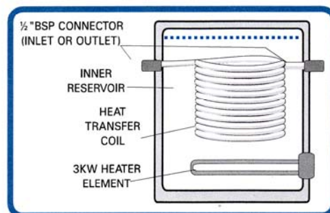
SCHEMATIC OF INTERIOR of COIL UDDER WASHER
